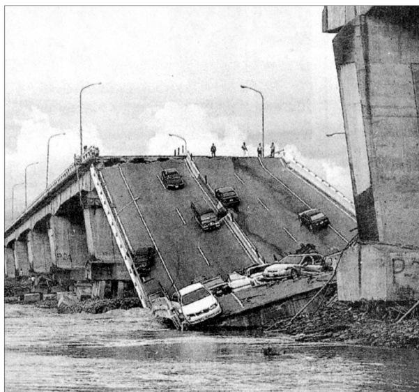
The Kaohsiung-Pingtung bridge, which collapsed yesterday
